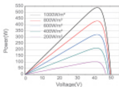
Power-Voltage Curve JAM72D30-540/MB
